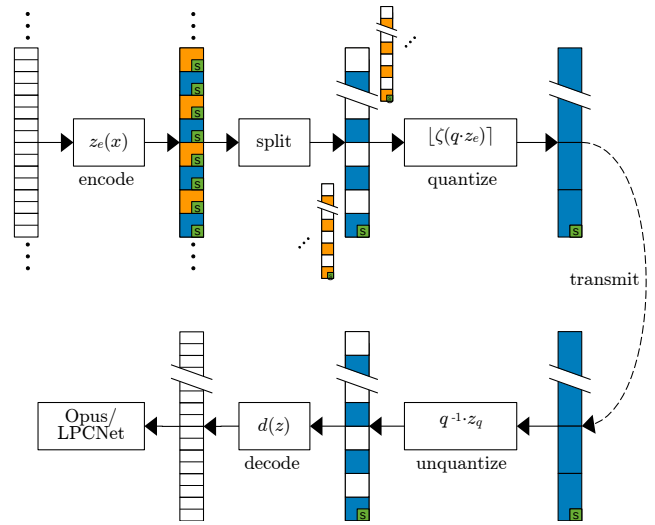
Fig. 2. Encoding and decoding process. The unquantized latent vectors are split into overlapping redundancy packets and then quantized using a variable resolution (the same vector can be quantized at different rates depending on its position). On the receiver, the redundancy packets are scaled back (unquantized), then decoded to produce 10-ms LPCNet feature vectors. The decoding process happens only on-demand such that no computation occurs when there is no loss.
