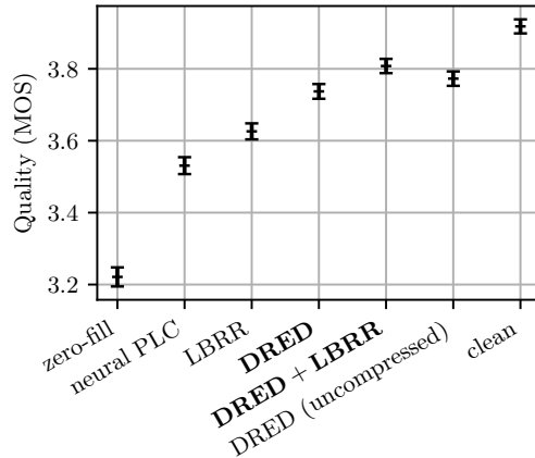
Fig. 3. MOS results, including the 95% confidence intervals. All differences are statistically significant.
